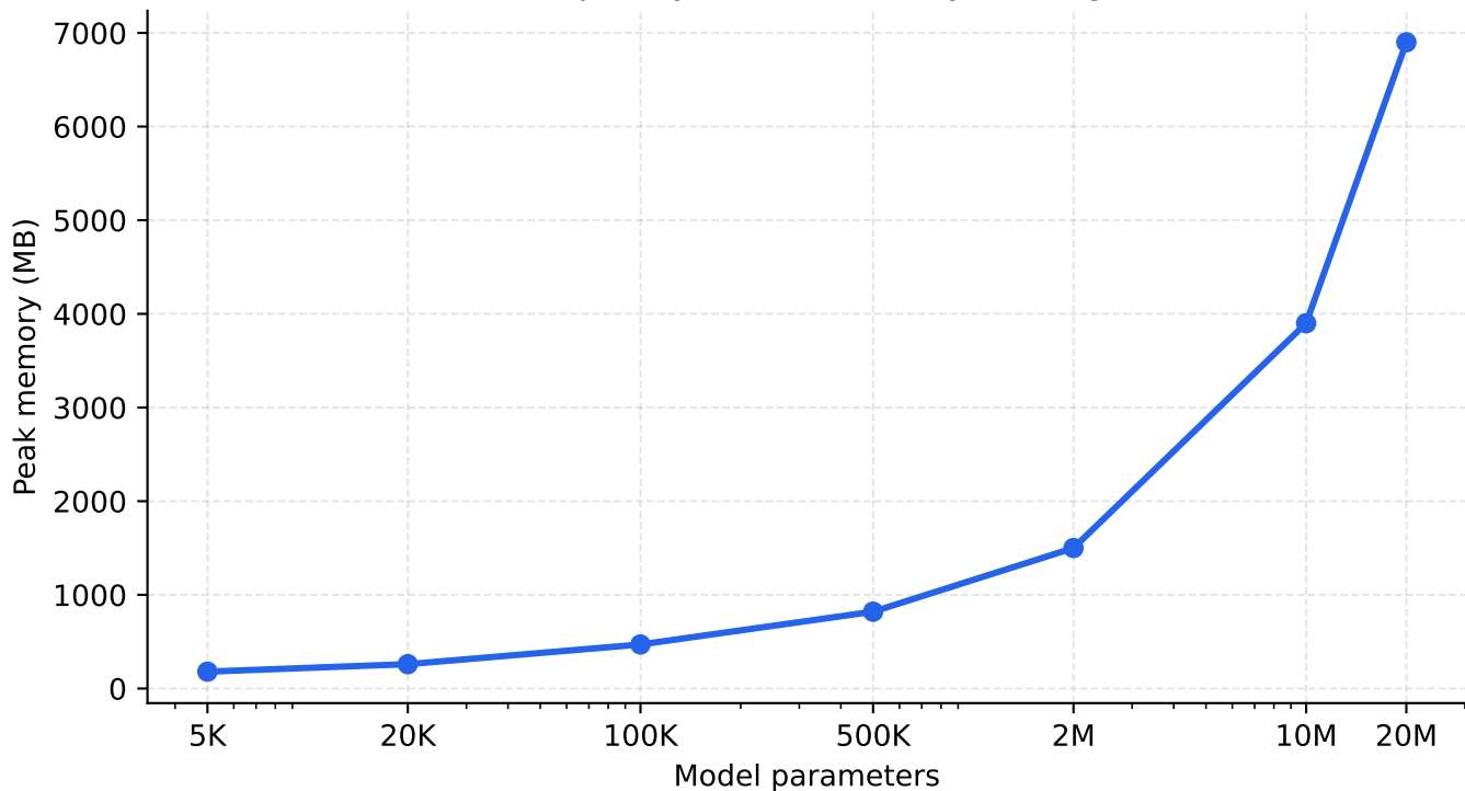
Temporary Solver Memory Scaling
