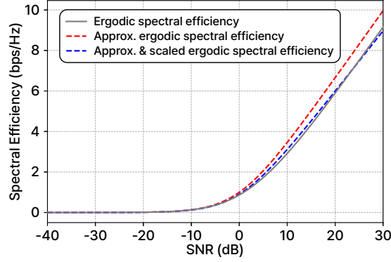
Fig. 13. Comparison between ergodic spectral efficiency and its approximation
