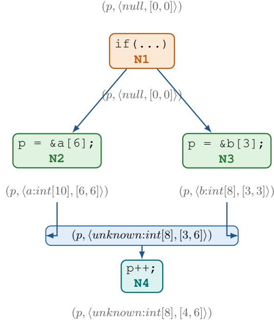
Figure 2: Control flow graph representing the C program segment of Fig. 1. Amber marks the branch node, green the pointer-assignment nodes, teal the pointer-arithmetic node, and blue the merged (safe) points-to-description computed at the join point.
