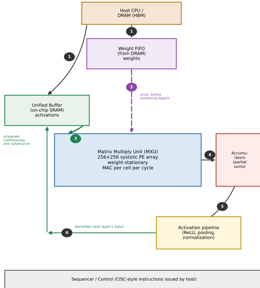
Data path for one layer of a neural network on a TPU-style accelerator
