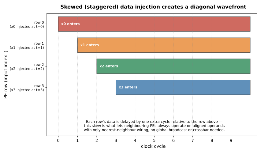
Figure 5: Staggering each row's injection by one extra cycle produces a diagonal wavefront: at any instant, exactly the PEs on one diagonal are doing meaningful work with correctly aligned data.
