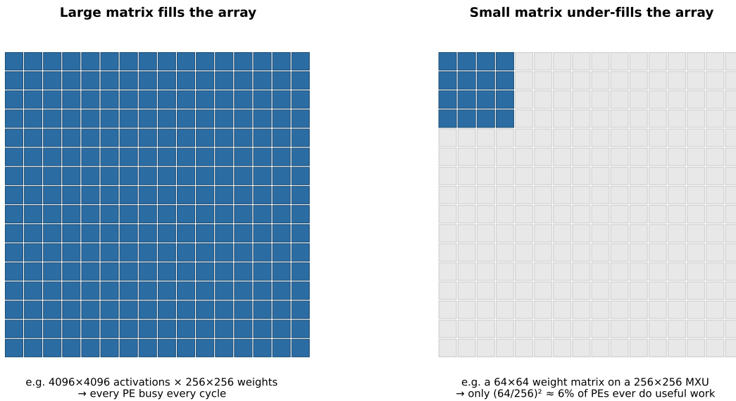
Figure 12: A matrix smaller than the array leaves most PEs idle every cycle — the same fixed mesh that gives perfect reuse on a well-matched problem gives poor utilization on a mismatched one.
