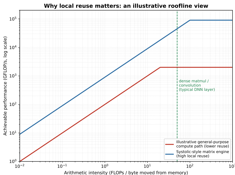
Figure 11: Illustrative roofline comparison. Local operand reuse can reduce memory traffic and increase effective arithmetic intensity, while a dedicated matrix engine can raise the peak-compute ceiling. Whether a particular matrix multiplication is memory- or compute-bound still depends on problem size, tiling, numerical format, bandwidth, and the memory hierarchy.
