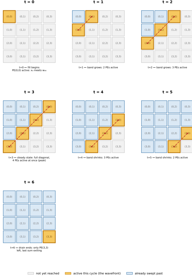
Figure 6: The same wavefront, viewed on the 4 \times 4 mesh from Figure 3, shown for every cycle from t = 0 to t = 6 . At each cycle, exactly the PEs with i + j = t are active (orange) — a diagonal band that enters at PE(0,0), grows one PE wider each cycle to its full width of 4 PEs at t = 3 , then shrinks back down to a single PE as it exits at PE(3,3).
