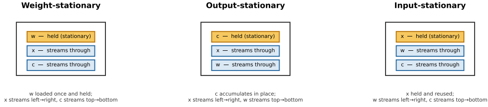
Figure 7: The three simple stationary dataflows illustrated with the same PE abstraction: weight-, output-, and input-stationary. Row-stationary, discussed in Table 1, is a more specialized convolution mapping and is not shown here, since it cannot be captured simply by pinning a different operand in this generic diagram.
