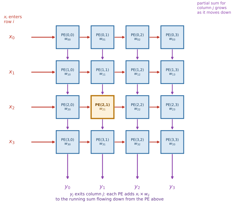
Figure 3: The identical layer, laid out as a 4 \times 4 systolic array. PE(i, j) permanently holds weight w_{ij} — the same w_{21} highlighted in Figure 2 sits in the highlighted PE(2, 1) here. Input x_i enters row i from the left; output y_j accumulates down column j and exits at the bottom.
