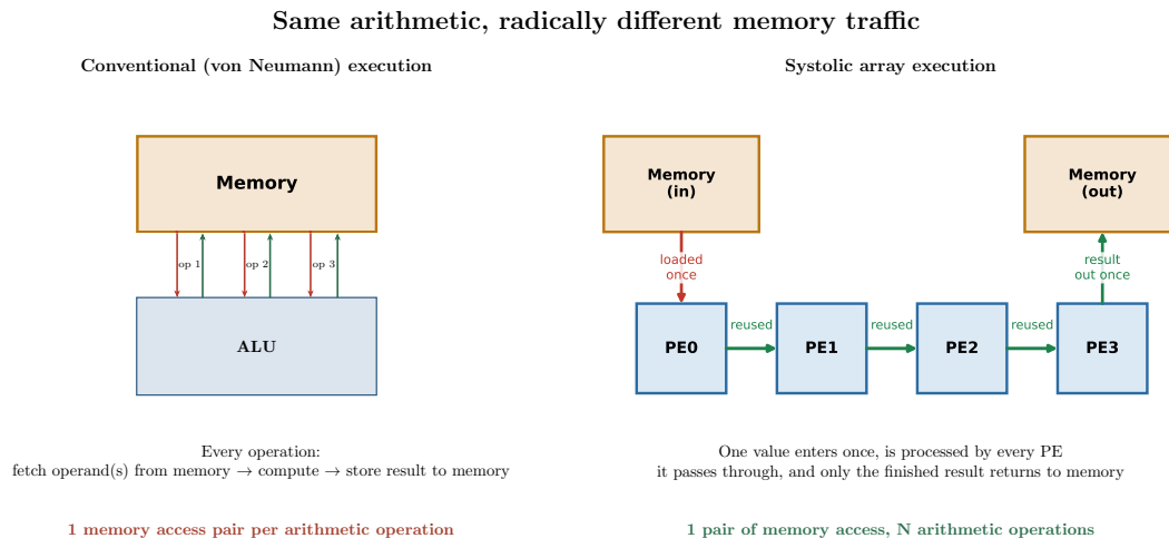
Figure 1: In a conventional design, memory is touched on every single operation. In a systolic array, a value is fetched from memory once and then reused by every PE it flows past before the finished result is written back — the whole point of the mesh is to turn memory accesses into a one-time cost instead of a per-operation cost.
