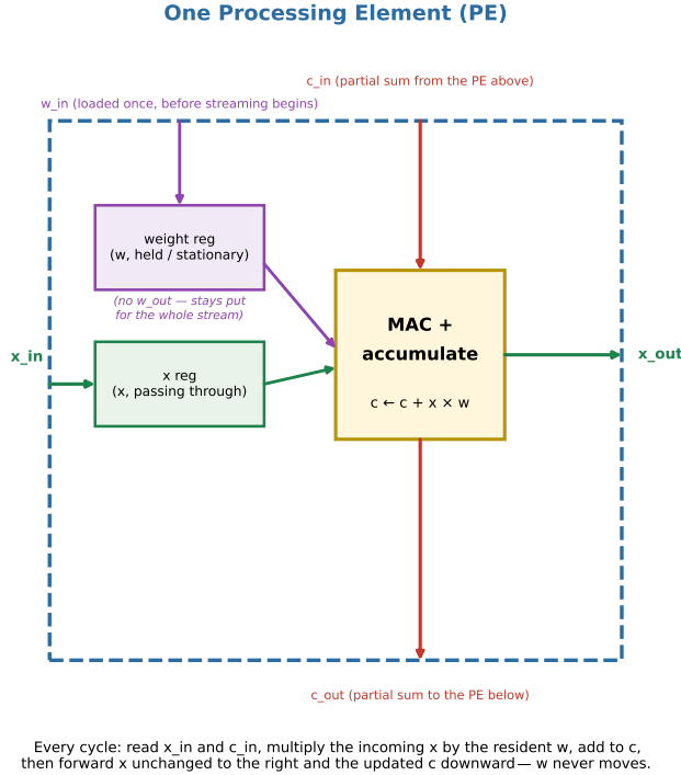
Figure 4: Internals of a single weight-stationary PE — concretely, PE(2, 1) from Figure 3. Its weight register holds w_{21} , loaded once and never moving; x_2 passes through unchanged on its way to PE(2, 2); the partial sum for column 1 is read in from PE(1, 1) above, updated by adding x_2 \times w_{21} , and pushed down to PE(3, 1).
