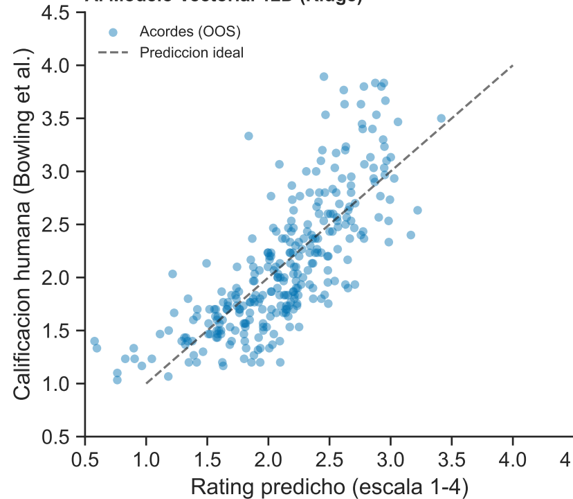
A. Modelo Vectorial 12D (Ridge)
