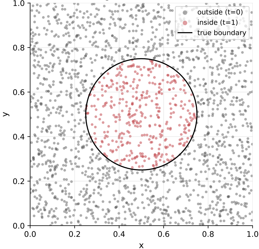
Circle data target (dense 2-22-1 learns this)
