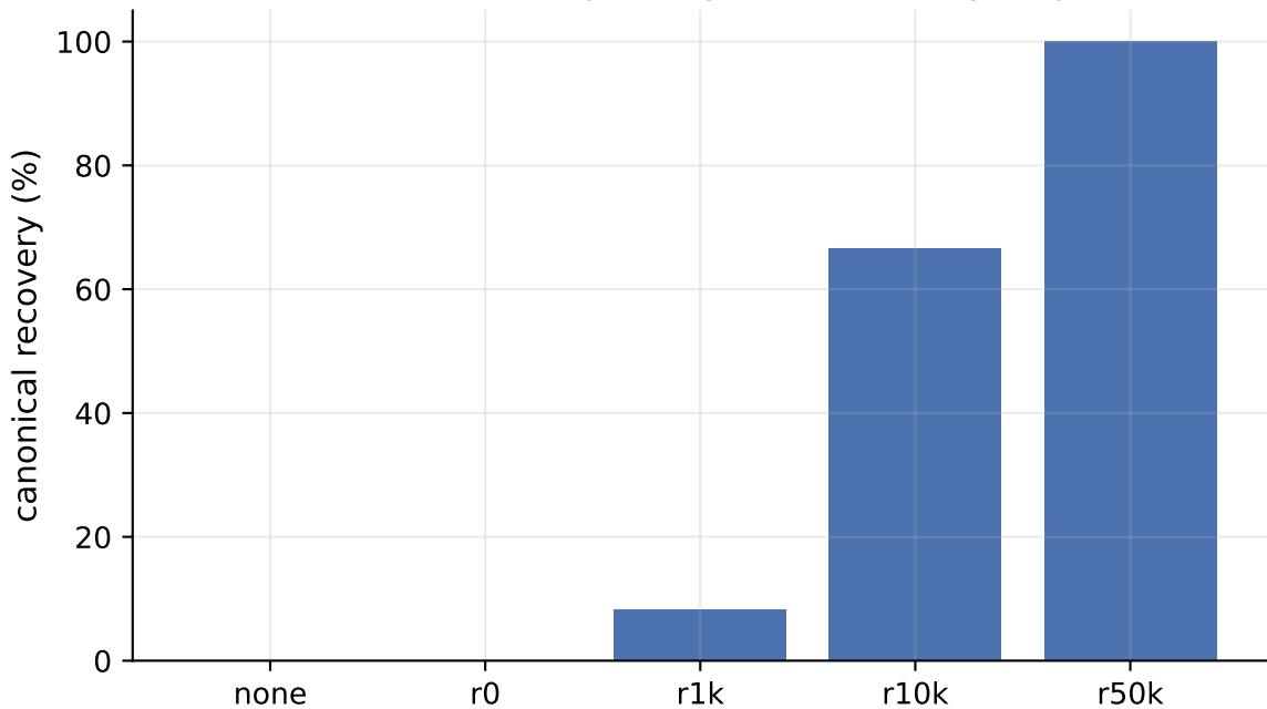
Canonical rate vs pruning/retrain setting (Exp08)
