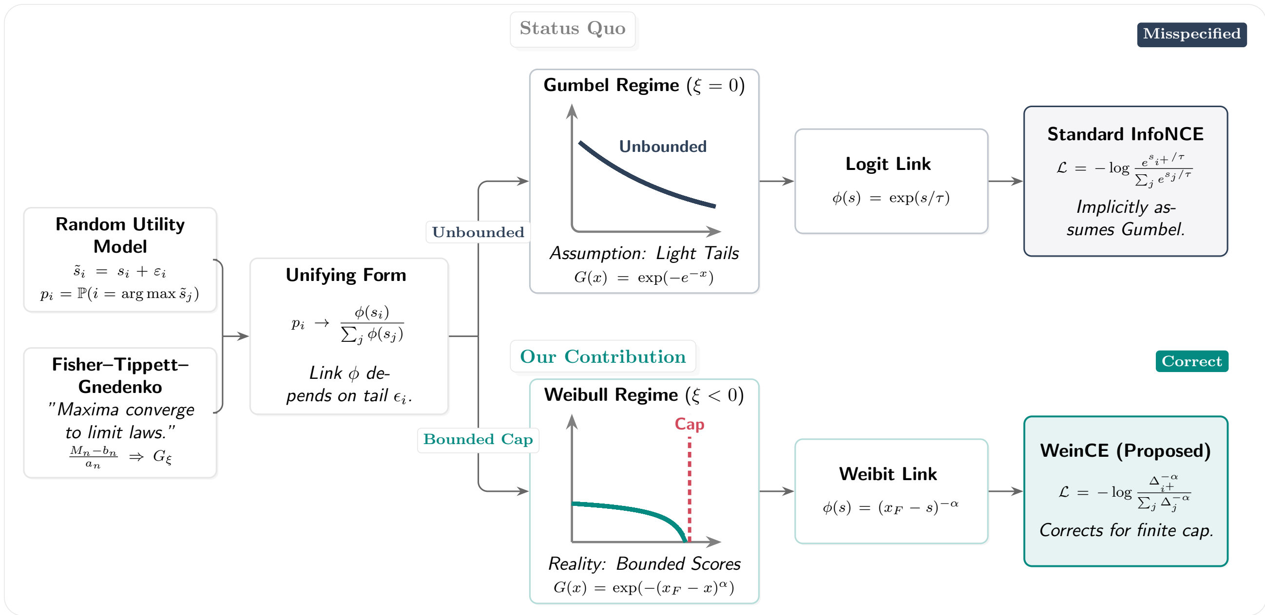
Figure 1: The WeinCE Framework. Left: Random Utility Modeling (RUB) and Extreme Value Theory (FTG) imply a Unifying Probability Form. Right: The induced link depends on the tail regime. Top row: the standard (Gumbel) assumption yields Logit and InfoNCE; bottom row: bounded scores (Weibull) yield the Weinbit link and our proposed WeinCE loss.
