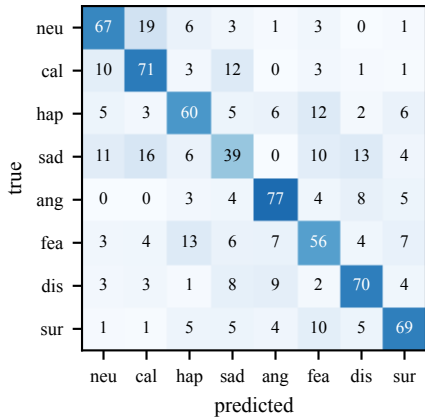
(a) ComParE + LR, UAR 63.6%
