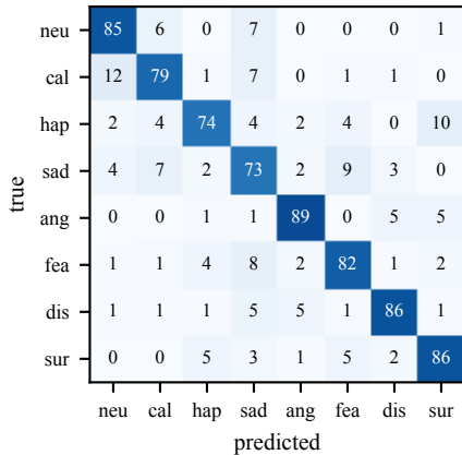
(b) XLS-R 300M + LR, UAR 81.9%
