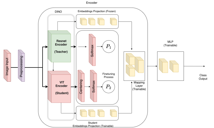
Fig. 1: Overview of DINO with ViT: The student network mimics the teacher output using two augmented views.
