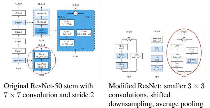
Fig. 5: Comparison of original and modified ResNet-50 stems to preserve spatial detail in early layers ((Red - Modified Block).
