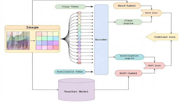
Fig. 4: Depiction of DeiT-III distillation token.
