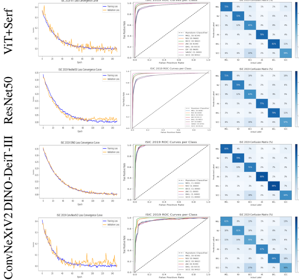
Fig. 10: ISIC 2019 dataset: Loss, ROC, and Confusion Matrix.
