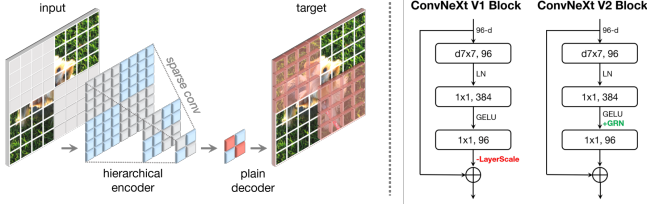
Fig. 6: ConvNeXtV2 block and hierarchical stage structure.
