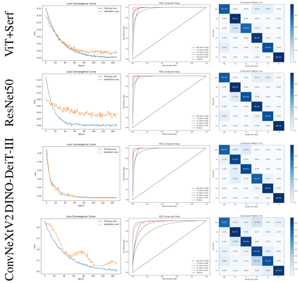
Fig. 8: CELLo dataset: Loss, ROC, and Confusion Matrix.
