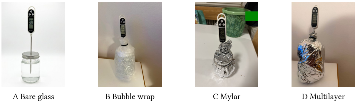
Figure 4. Standard four-configuration comparison assemblies.
