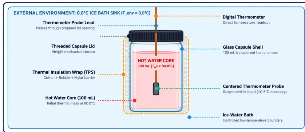
Image A. Final capsule arrangement showing the warm-water core, centred probe, insulation wrap, and ice-water boundary.
