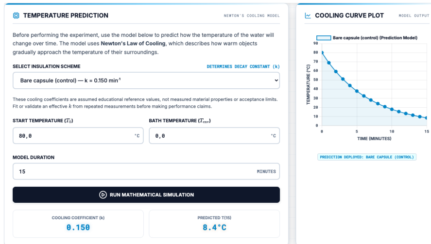
Image C. Current Mission Control prediction interface and 15-minute cooling curve.
