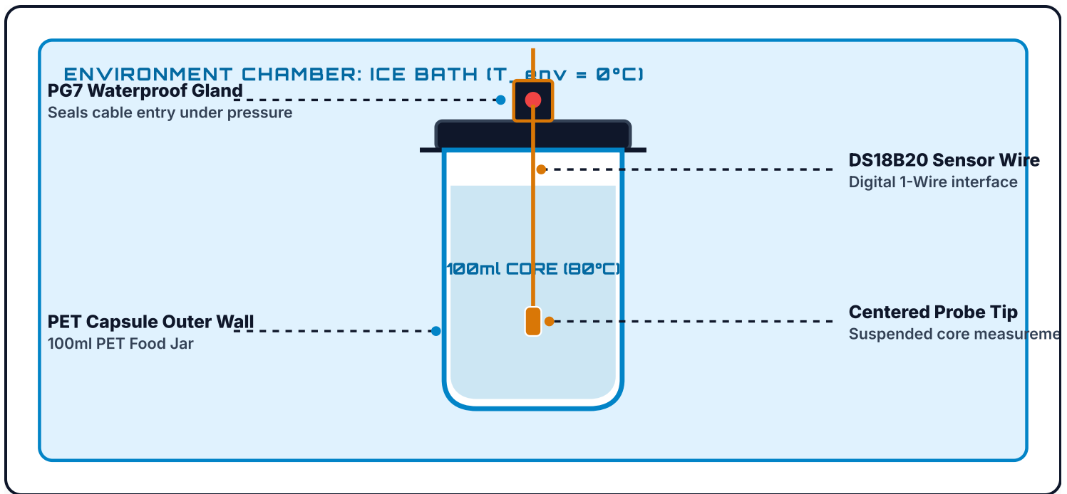
FIGURE 1: MECHANICAL ASSEMBLY DIAGRAM & THERMAL PROBE SEEDING
