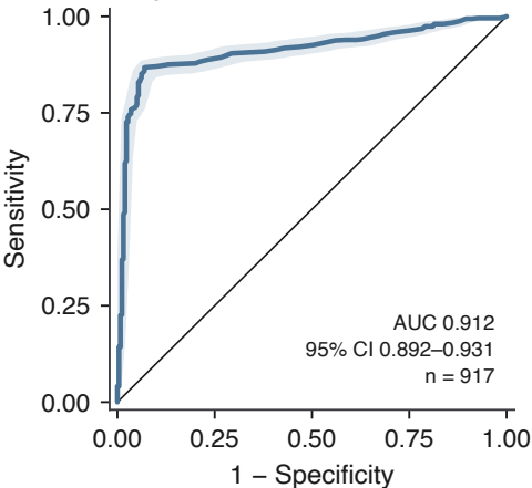
Stage 1 — Gatekeeper
