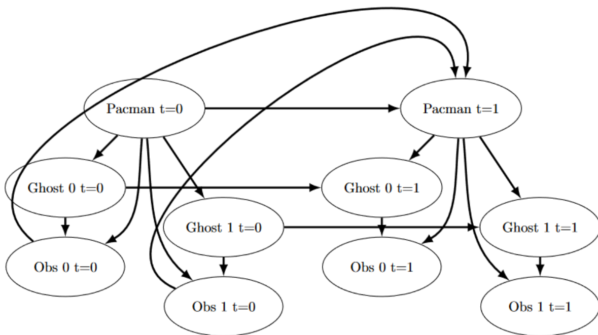
Bayes net diagram
