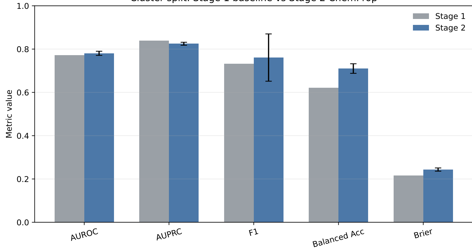
Cluster split: Stage 1 baseline vs Stage 2 ChemProp
