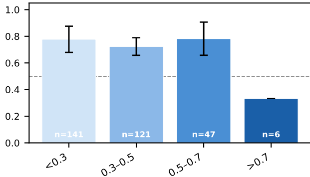
XGBoost
