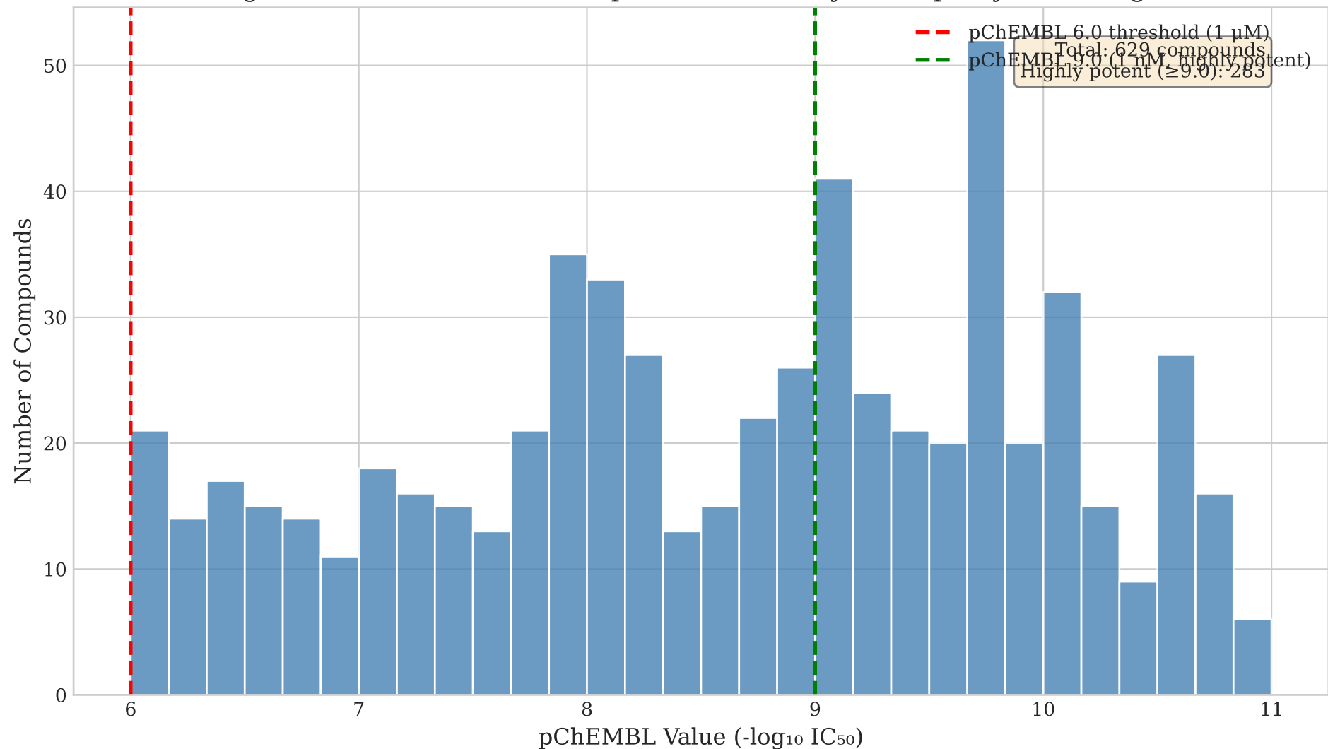
Figure 2: Distribution of Compound Bioactivity for Leprosy HDT Targets
