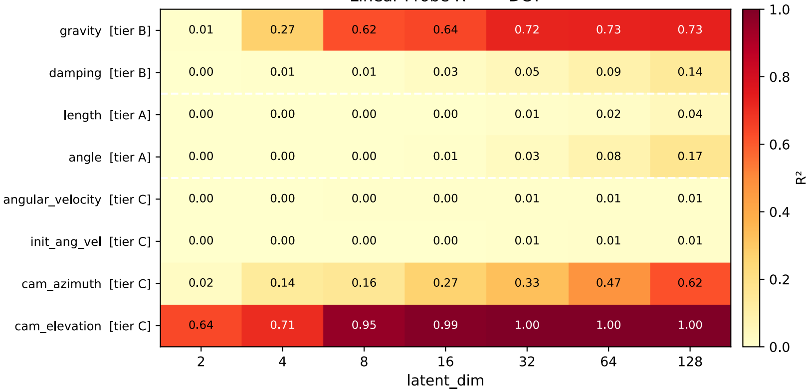
Linear Probe R 2 — DCT
