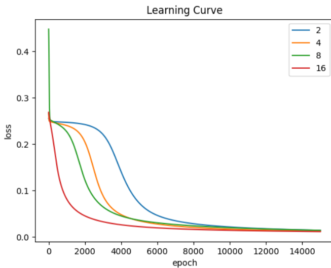
(a) Linear
