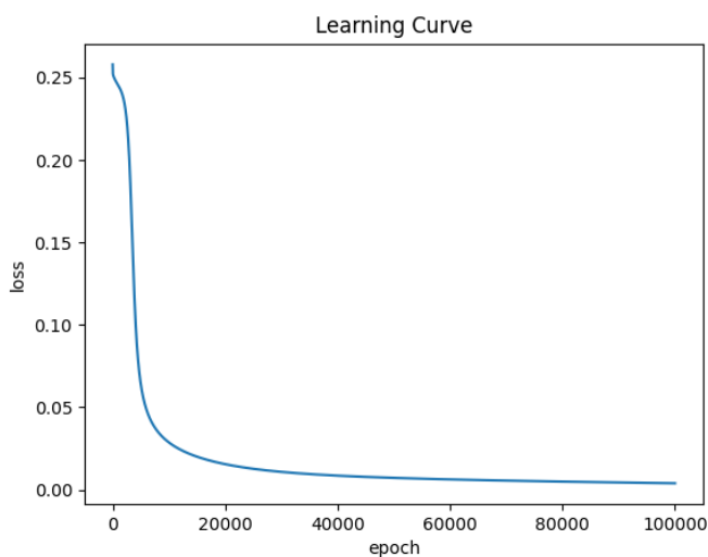
(a) Linear
