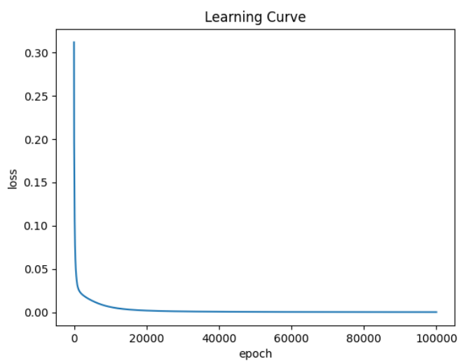
(a) Linear
