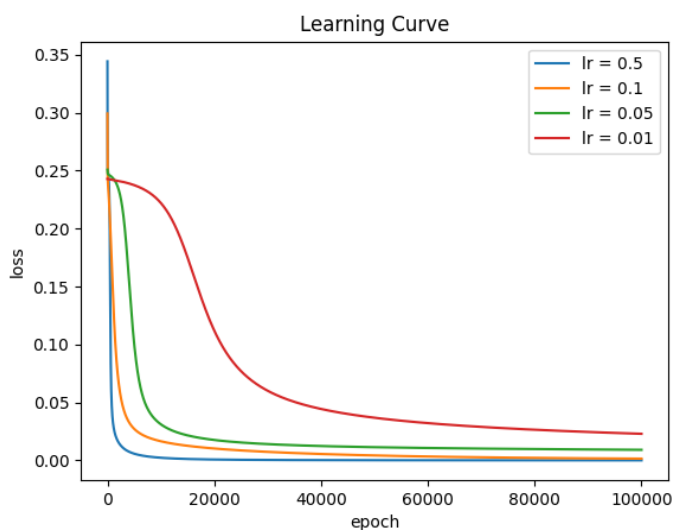
(a) Linear
