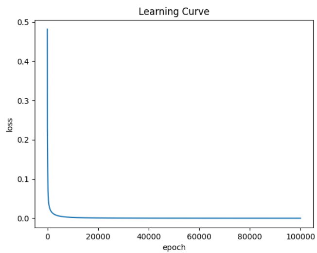
(a) Linear
