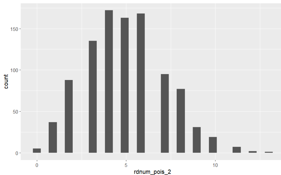
Figure: Random Samples with size 1000 drawn from \text{Poisson}(\lambda = 5)
