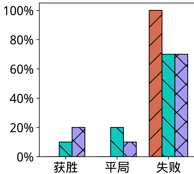
naiveMCTSAI
