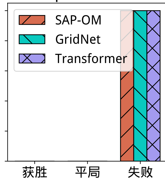
passiveAI
