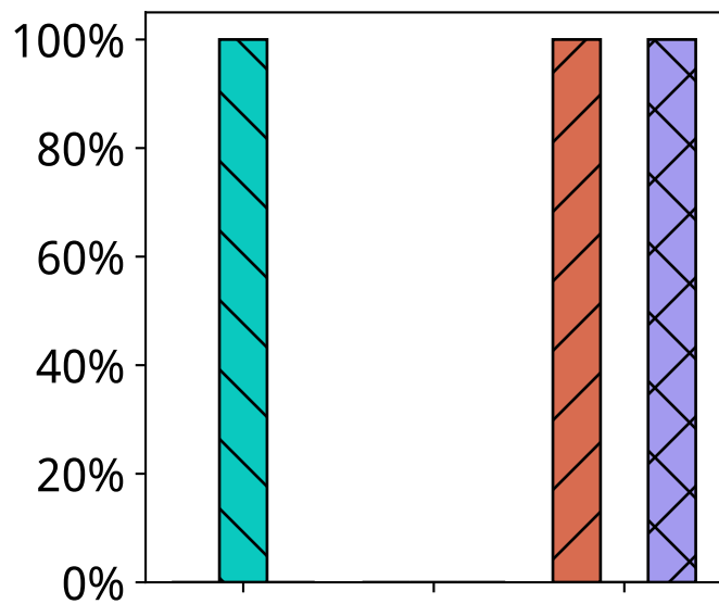
coacAI
