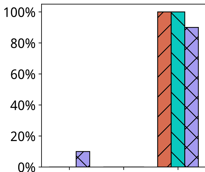
mixedBot
