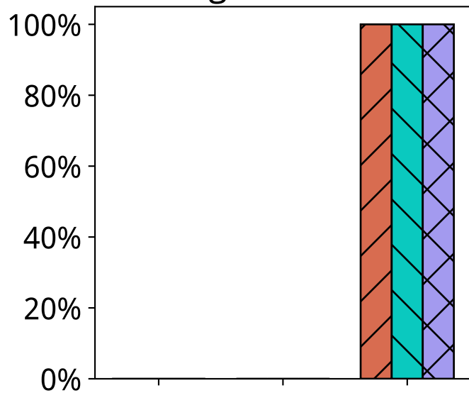
lightRushAI
