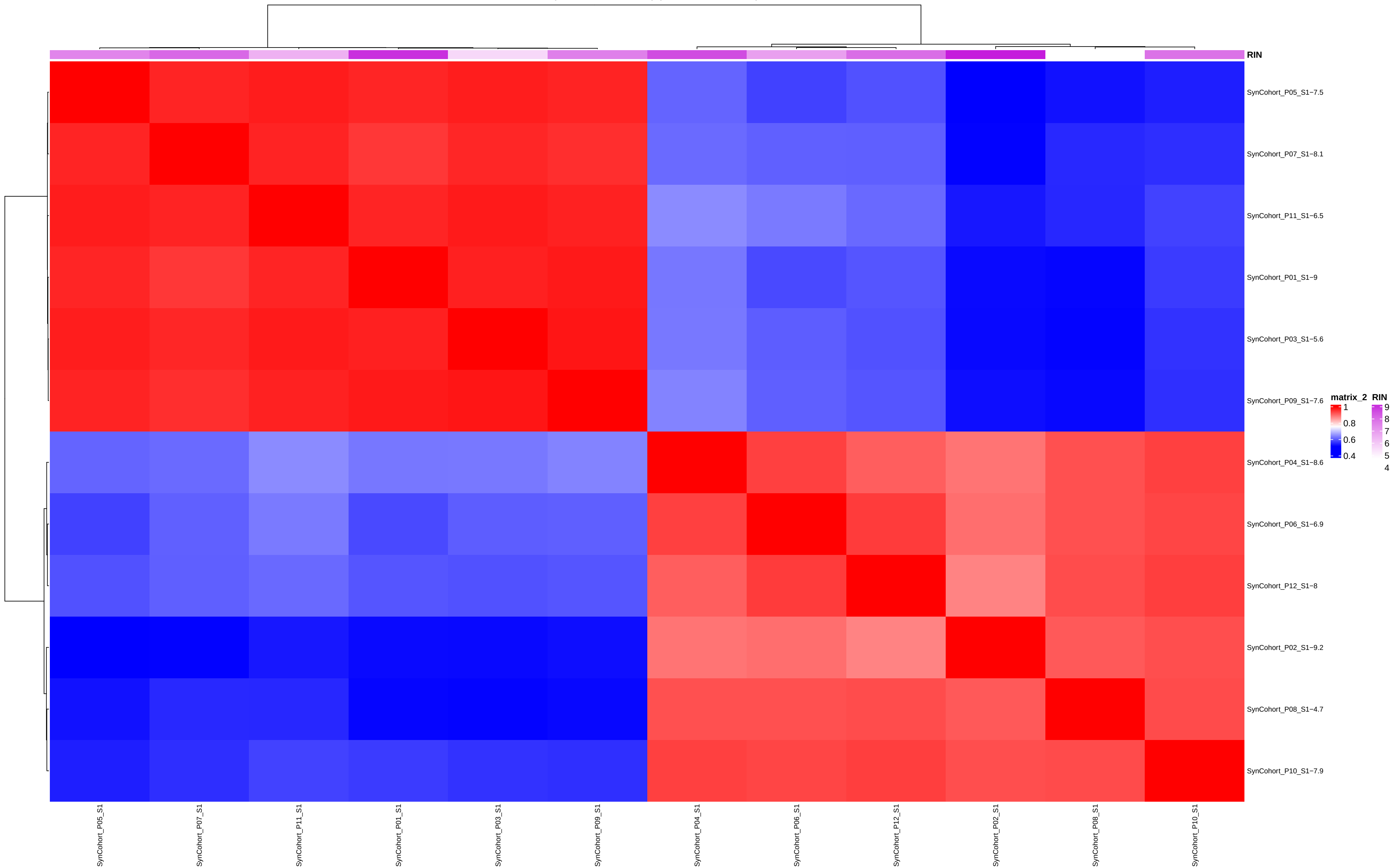
Sample Correlation Heatmap (RIN Median Annotated)
