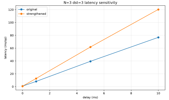
Fig. 3. Per-operation latency for N = 3 , \text{dst}=3 under artificial protocol-message delay.
