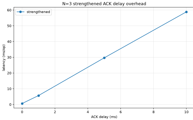
Fig. 4. Per-operation latency for N = 3 , dst=3 when artificial delay is applied only to ACK messages.
