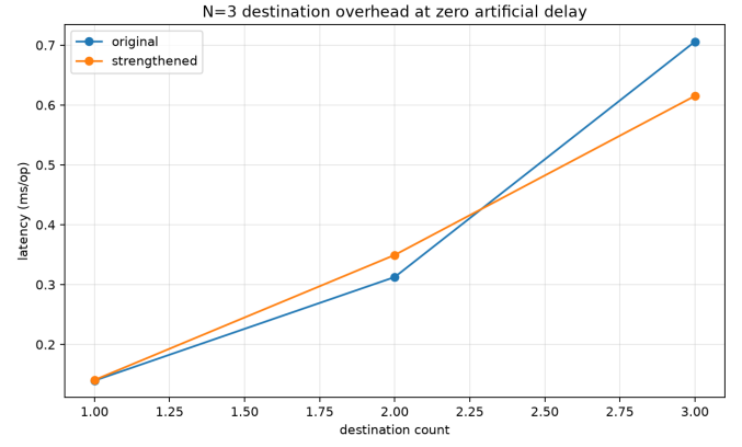
Fig. 2. Destination-set overhead for N = 3 without artificial latency.
