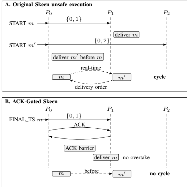
Fig. 1. Conceptual sequence diagram for the reproduced unsafe execution. In original Skeen, a real-time edge m \rightarrow m' can coexist with a delivery-order edge m' \rightarrow m at an overlapping destination, forming a cycle. The ACK-gated variant delays delivery until all destinations acknowledge the final timestamp, preventing the premature delivery used by the counterexample.
