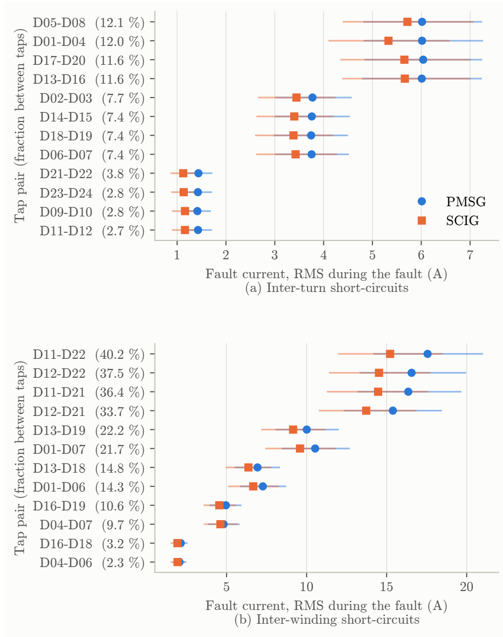
Fig. S1 Fault current per tap pair, PMSG and SCIG, for inter-turn (a) and inter-winding (b) short-circuits: mean over the nine operating points (marker) and range (bar). Rated currents 6.3 A (PMSG) and 7.7 A (SCIG)
