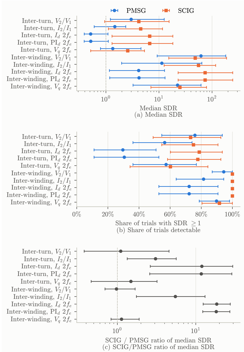
Fig. S2 Tap-pair-level uncertainty: bootstrap 95% intervals of the median SDR (a), the detectable share (b) and the SCIG/PMSG ratio of median SDR (c) for five features and both fault classes (the same resampled tap pairs for both machines), five-cycle windows
