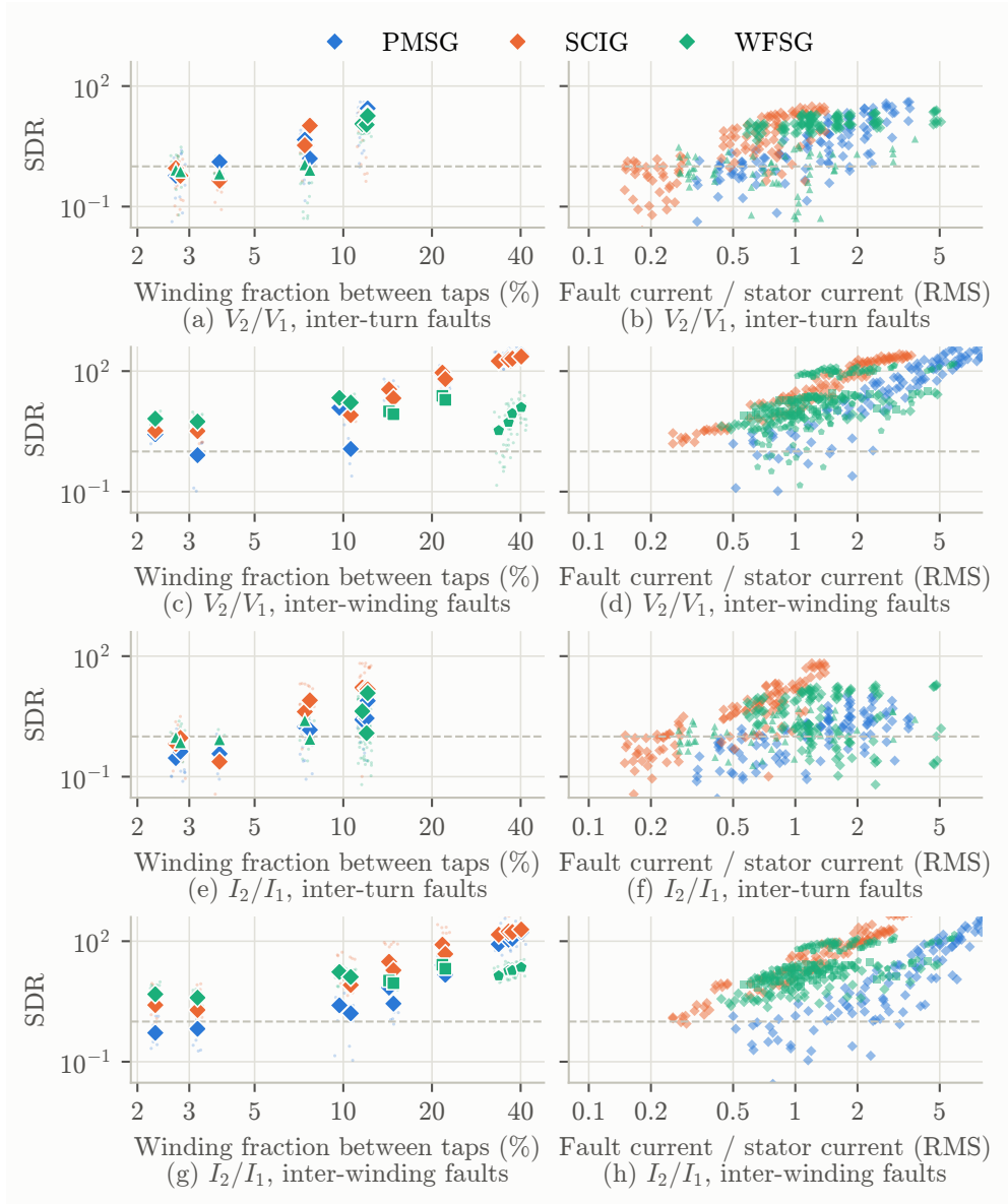
Fig. 3 Signal-to-drift ratio of V_2/V_1 (a–d) and I_2/I_1 (e–h) for the three alternatives, three-cycle windows, against the design-level fault extent (left column; small dots: trials; large markers: median per extent level and fault impedance, marker shape encoding the impedance) and against physical fault severity (right column; RMS fault current relative to the RMS pre-fault stator current, all trials)
