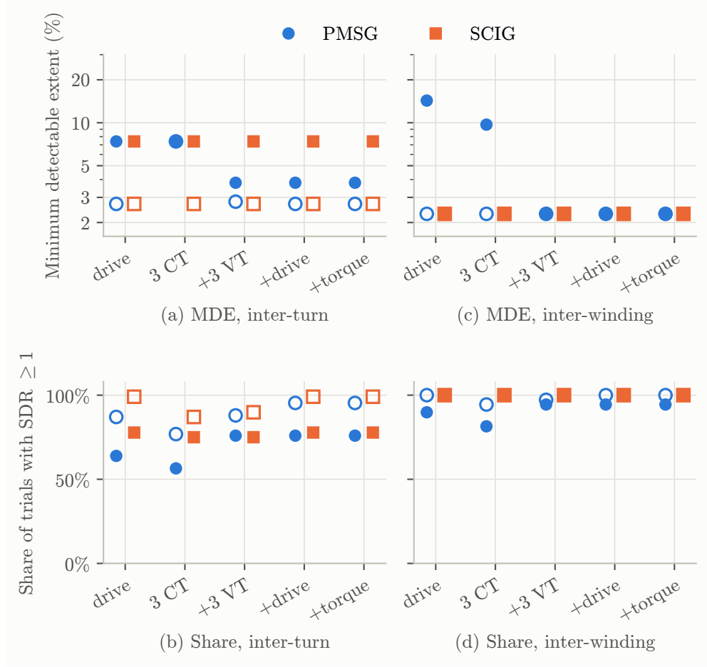
Fig. 4 Observation suites versus what they detect, PMSG and SCIG (five-cycle windows): minimum detectable extent (MDE; a , c ) and detectable share ( b , d ) for the fixed best feature of each suite (filled; the feature is named in Table 6) and the per-trial oracle (hollow)
