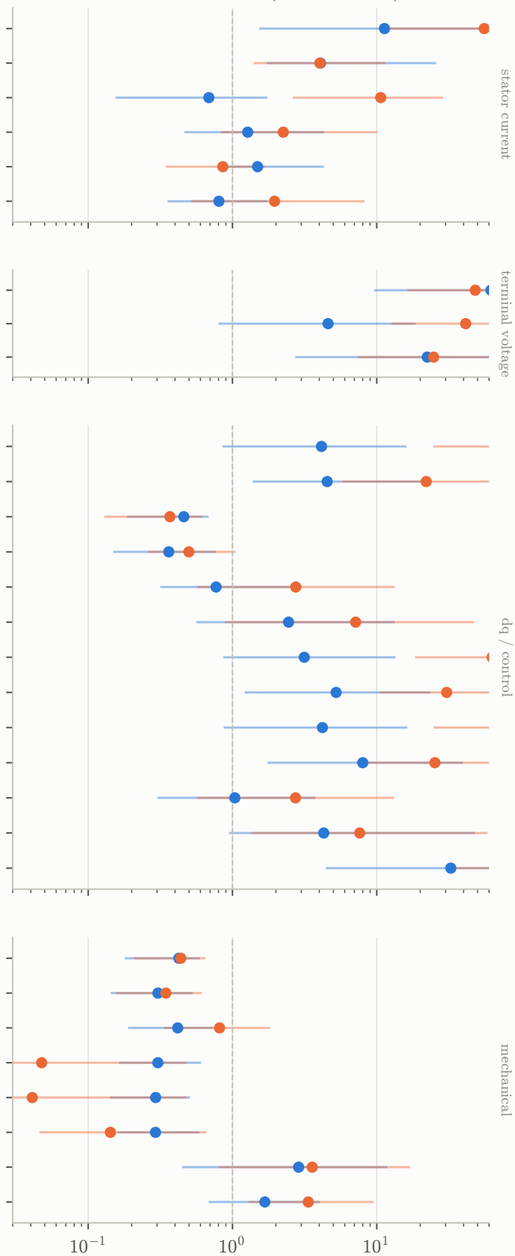
Inter-winding faults (108 recordings)
