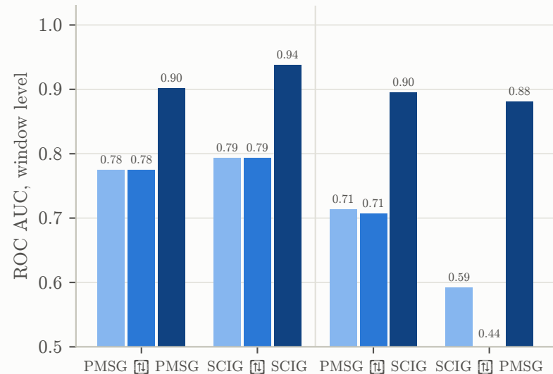
logistic classifier
