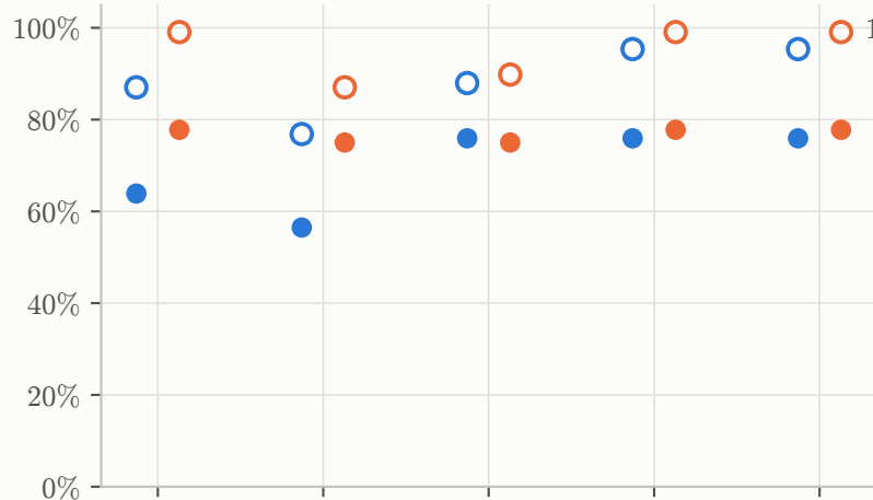
Share of fault recordings detectable ( \text{SDR} \geq 1 )
