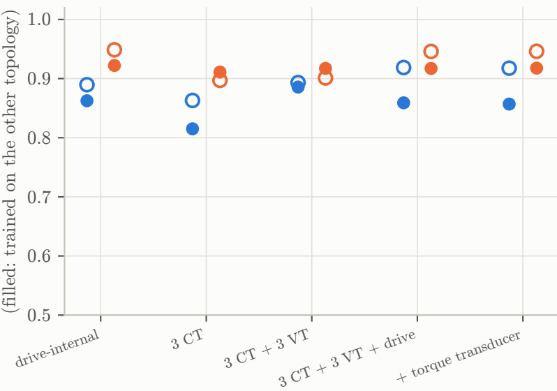
features as —z— vs own pre-fault segment
