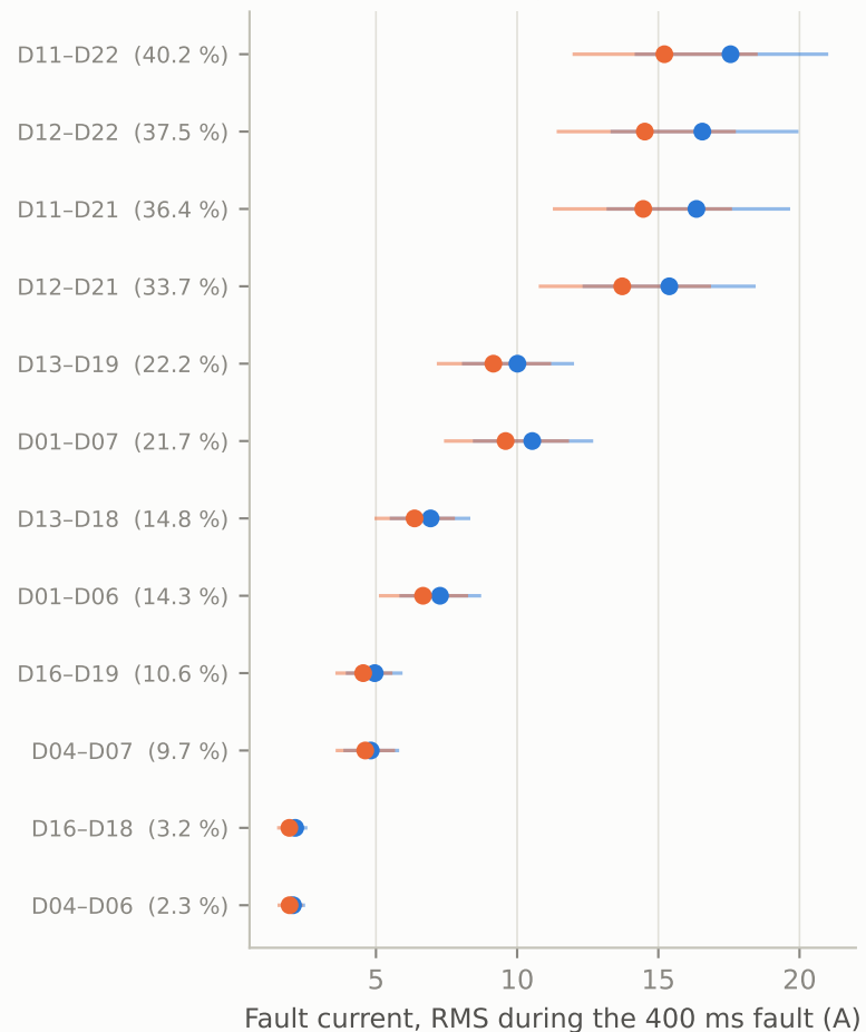
Inter-winding short-circuits
