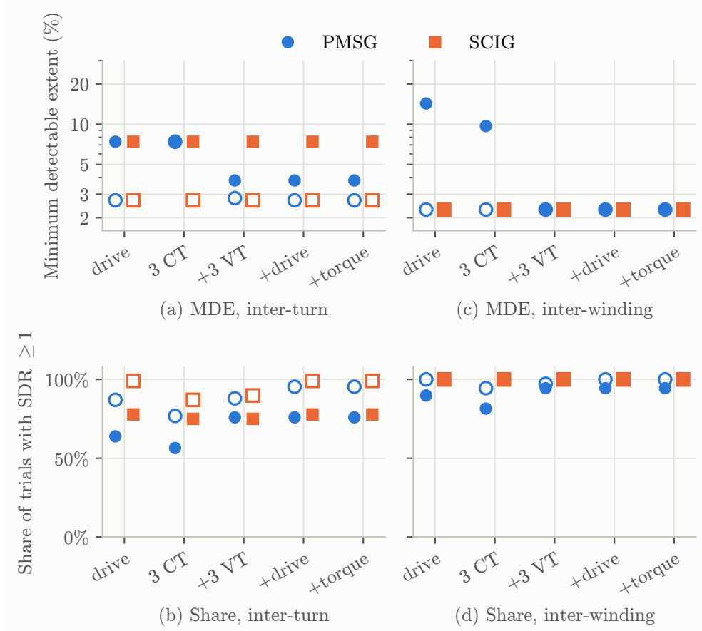
Fig. 4 Observation suites versus what they detect, PMSG and SCIG: MDE (a, c) and detectable share (b, d) of the fixed best feature (filled) and the per-trial oracle (hollow)
