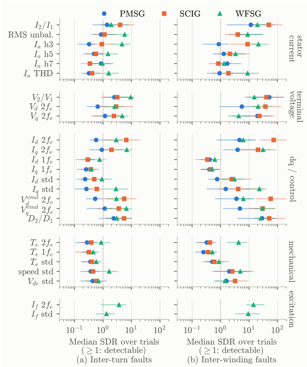
Fig. 2 Median SDR of every feature (dot) with interquartile range (bar) for the three alternatives, three-cycle windows
