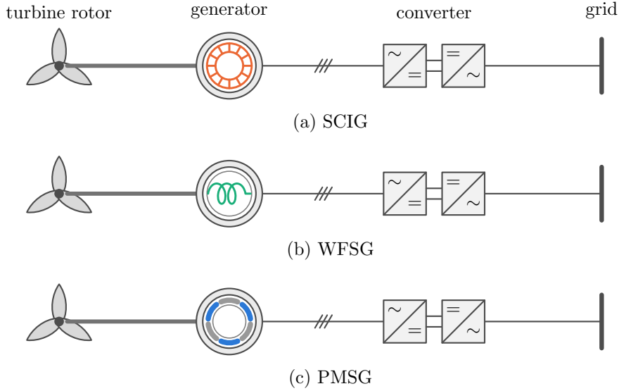
Fig. 2 The three alternatives as generator systems: turbine rotor, generator with its rotor excitation (squirrel cage, field winding, permanent magnets), back-to-back converter and grid
