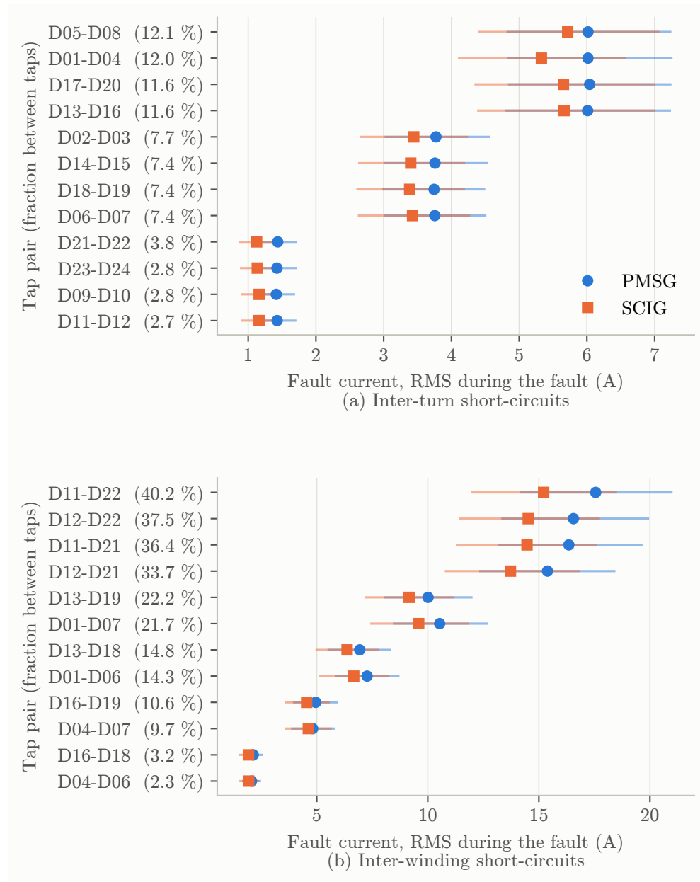
Fig. S1 Fault current per tap pair, PMSG (rated 6.3 A) and SCIG (7.7 A), inter-turn (a) and inter-winding (b) faults: mean over the nine operating points (marker) and range (bar)
