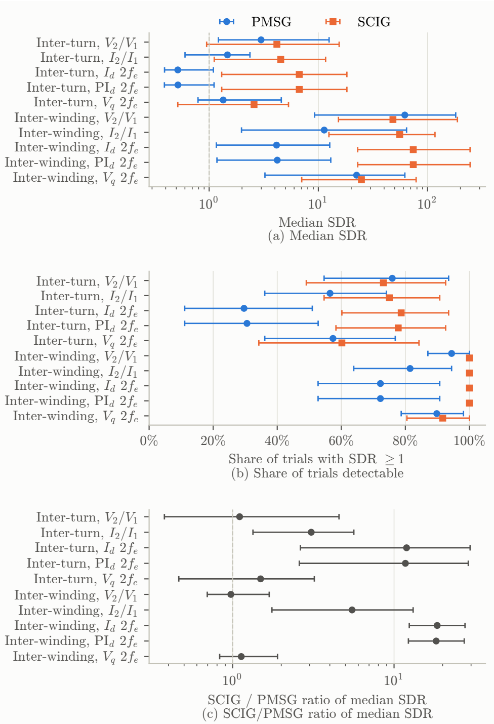
Fig. S2 Tap-pair bootstrap 95% intervals of the median SDR (a), the detectable share (b) and the SCIG/PMSG ratio of median SDR (c), five-cycle windows
