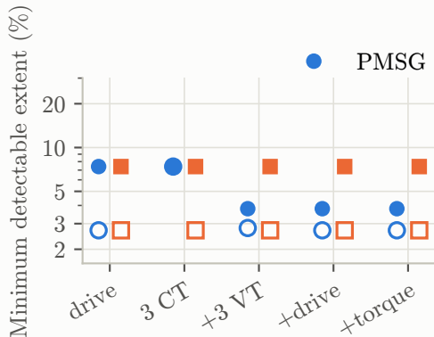
(a) MDE, inter-turn
