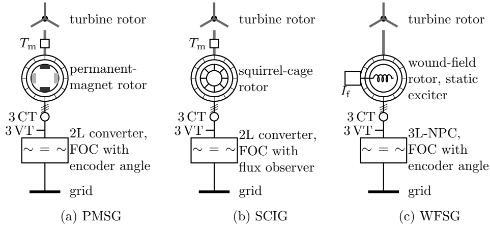
Fig. 2 The three alternatives: rotor excitation, converter and control, with the measurement points of the observation suites (3 CT, 3 VT, T_m , I_f )
