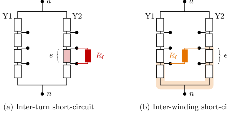
Fig. 3 Inter-turn (a) and inter-winding (b) short-circuits through R_f between taps of one phase of the double-star stator (schematic); e is the fraction of a branch between the taps
