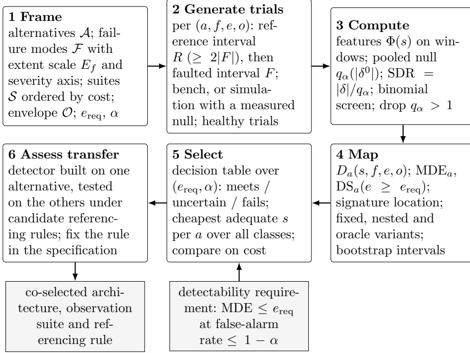
Fig. 1 The design procedure. Steps 3–4 are fully specified by Eqs. (1)–(2); steps 1, 2, 5 and 6 are design decisions for which Section 3.4 gives default rules
