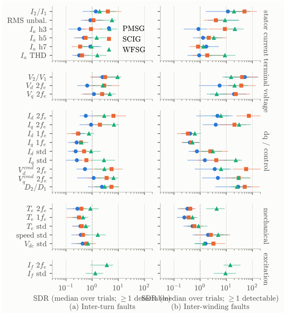
Fig. 2 Median signal-to-drift ratio of every feature for the three alternatives (dot) with interquartile range (bar), three-cycle windows; features to the right of the dashed line are detectable in more than half of the trials. The WFSG rows pool all its fault impedances
