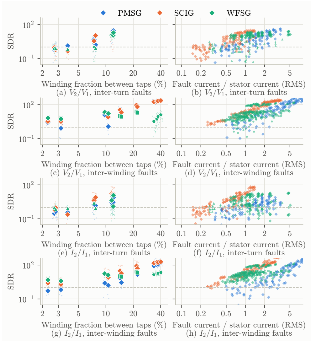
Fig. 3 Signal-to-drift ratio of V_2/V_1 (a–d) and I_2/I_1 (e–h) for the three alternatives, three-cycle windows, against the design-level fault extent (left column; small dots: trials; large markers: median per extent level and fault impedance, marker shape encoding the impedance) and against physical fault severity (right column; RMS fault current relative to the RMS pre-fault stator current, all trials)
