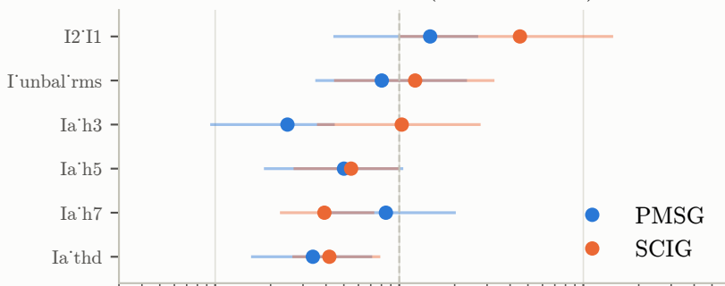
Inter-turn faults (108 recordings)
