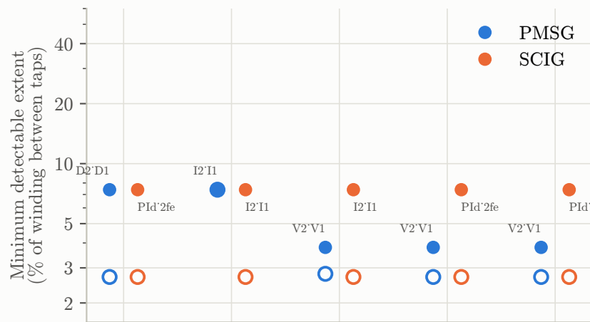
Inter-turn faults
