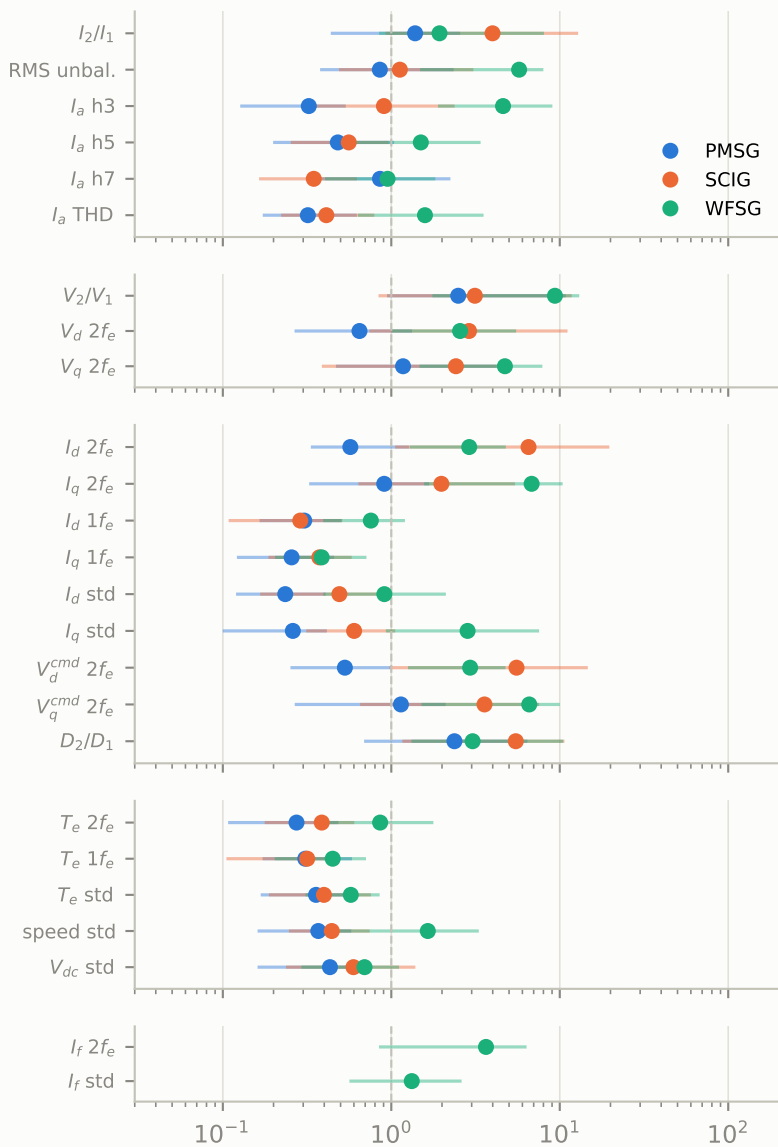
Inter-turn faults
