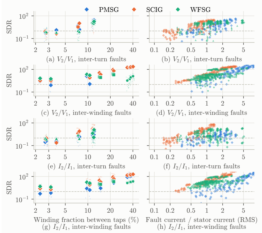
Fig. 5 SDR of V_2/V_1 (a–d) and I_2/I_1 (e–h) against the design-level extent (left) and the physical severity (right), three alternatives, three-cycle windows
