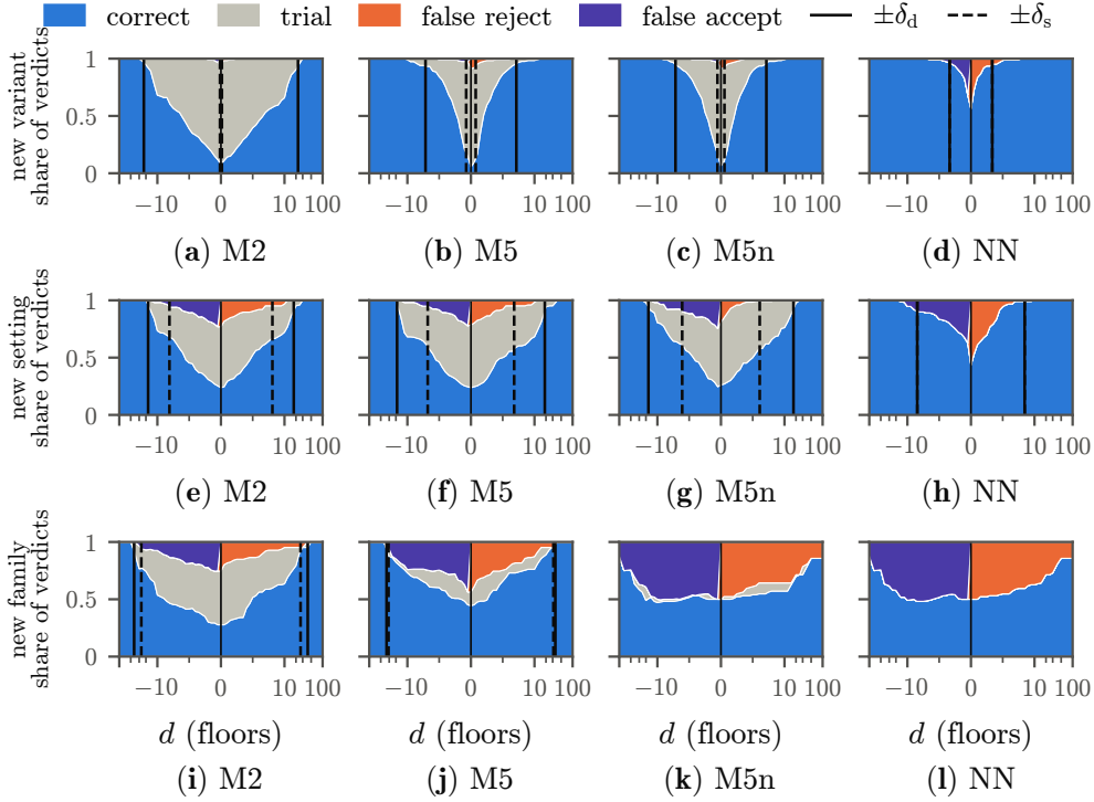
Fig. 2 Verdict shares against the requirement distance d (symmetric logarithmic axis, linear within \pm 10 floors; 126 cases per panel; a new family in the produced family's floor), with \delta_d and \delta_s
