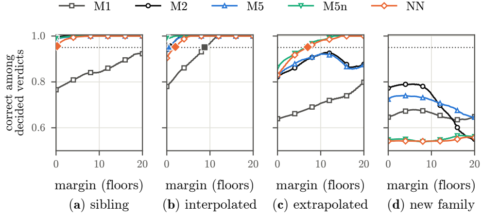
Fig. 4 Share correct among decided verdicts with at least the given margin; reference prior: 47 grid distances within \pm 20 floors, equal weights; new family in the produced family's floor; filled markers: g
