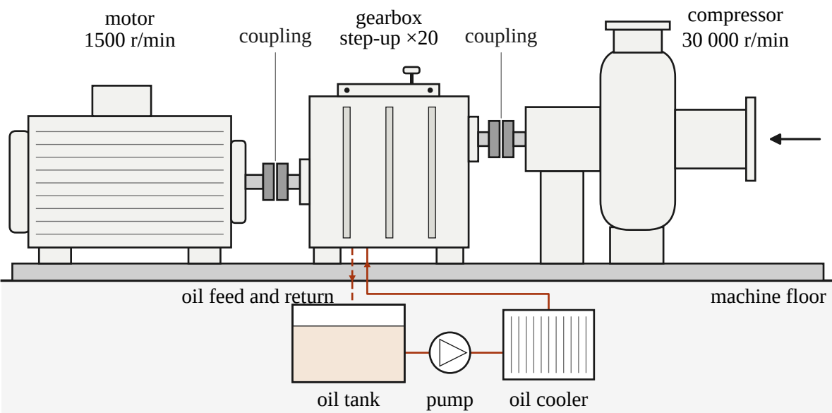
(a) Geared train
