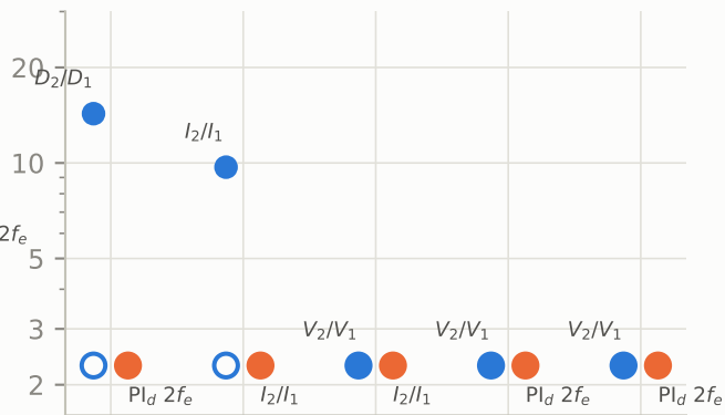
Inter-winding faults
