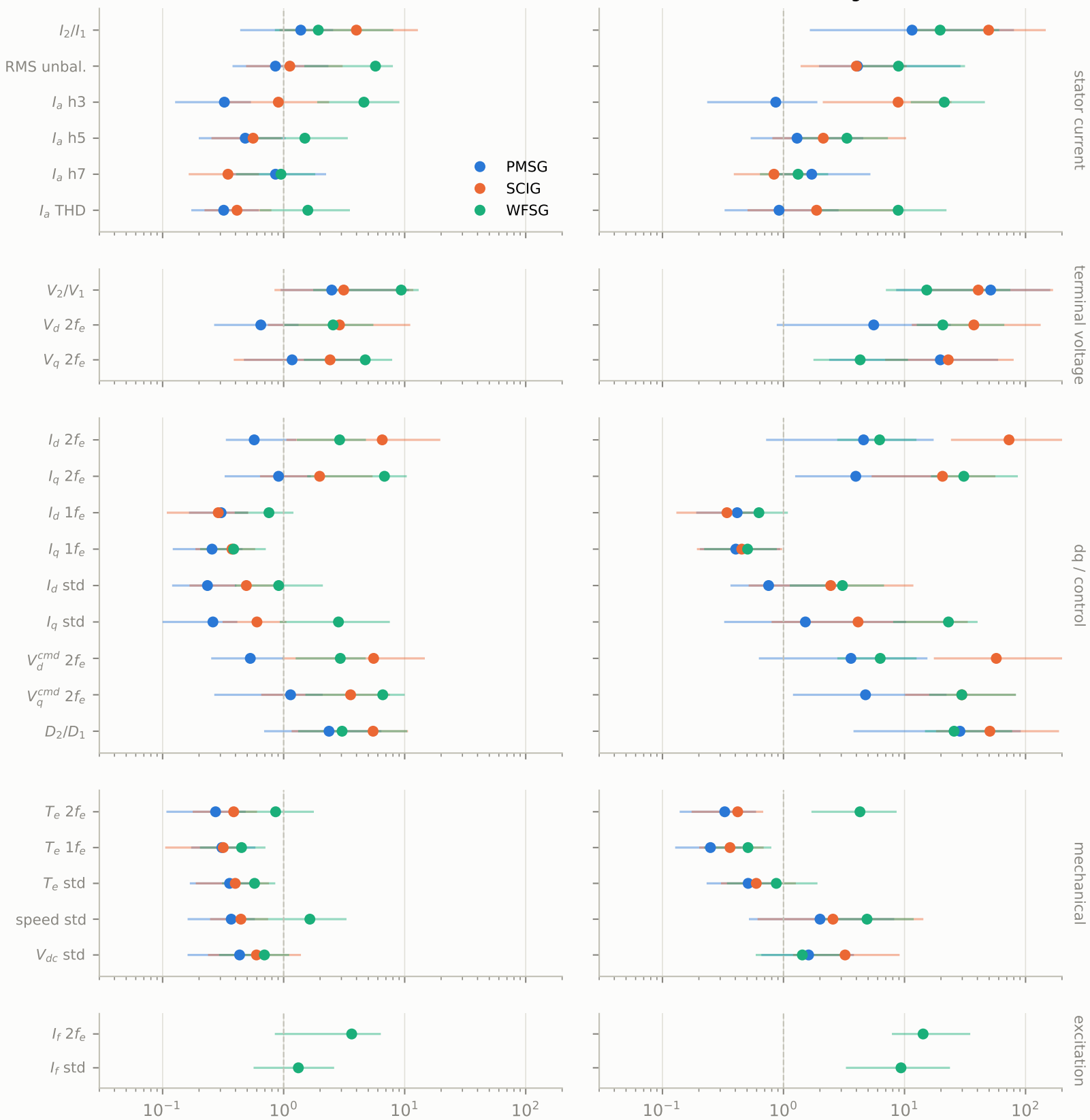
Inter-turn faults
