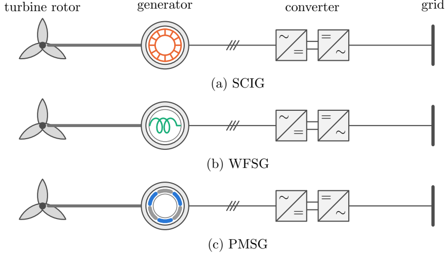
Fig. 2 The three alternatives as generator systems: turbine rotor, generator with its rotor excitation (squirrel cage, field winding, permanent magnets), back-to-back converter and grid
