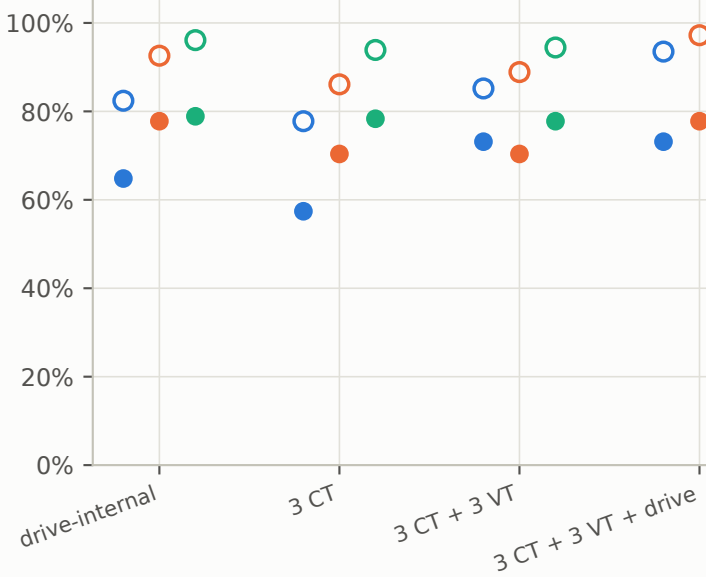
Share of fault recordings detectable ( \text{SDR} \geq 1 )
