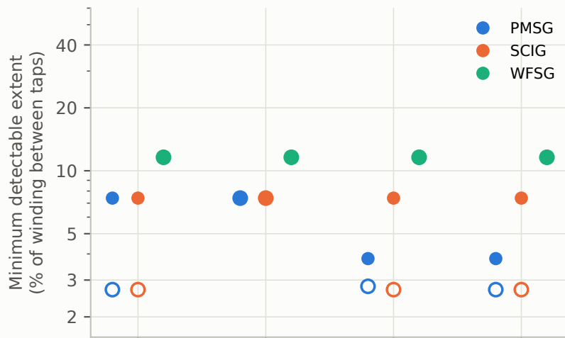
Inter-turn faults
