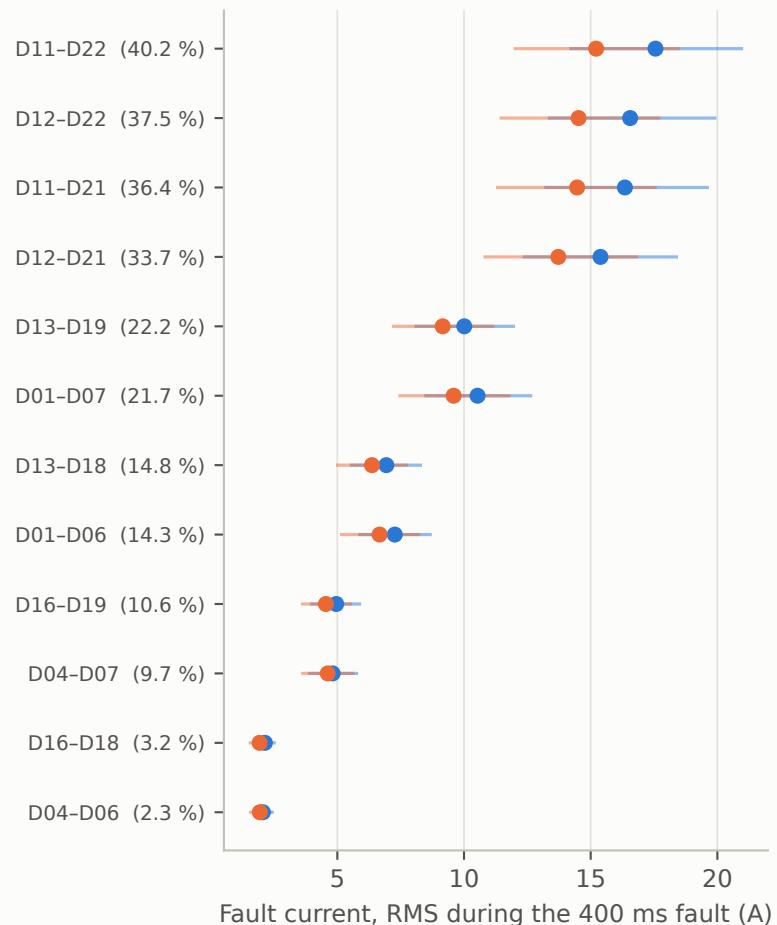
Inter-winding short-circuits
