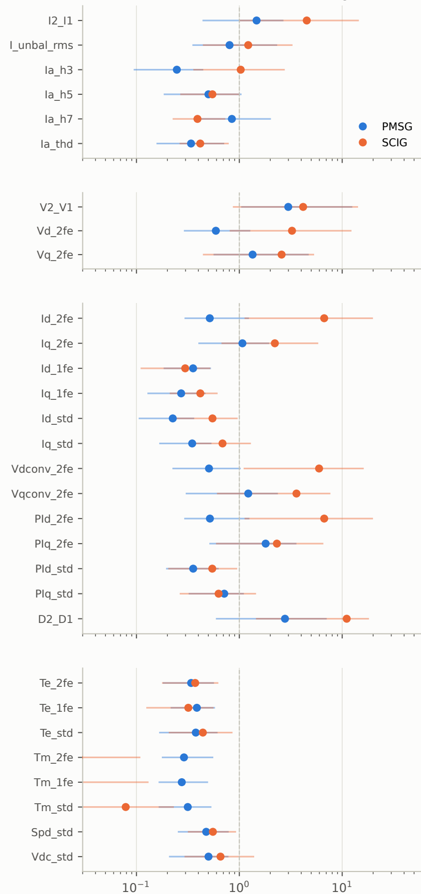
Inter-turn faults (108 recordings)
