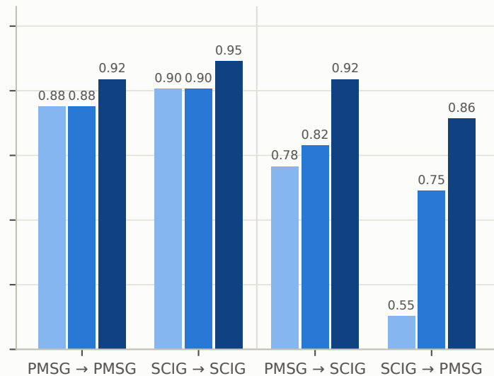
gbdt classifier
