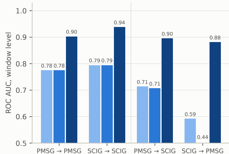
logistic classifier
